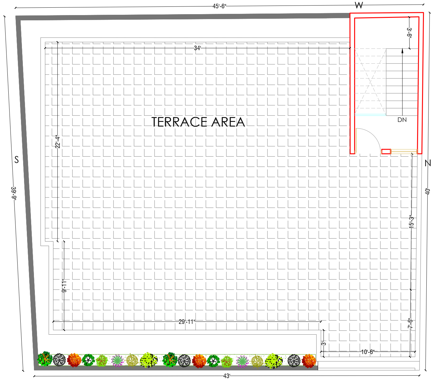
TERRACE FLOOR PLAN :- 127 SFT
